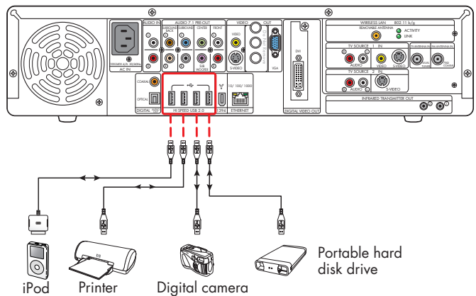
USB device connection (back panel)
